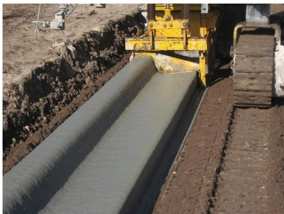
Figure 19.8 – Kerb Construction 19.3
