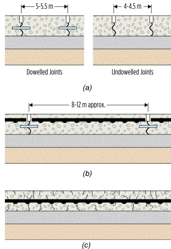
Figure 19.5 – (a) PCP; (b) JCRP; (c) CRCP
