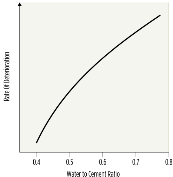
Figure 25.29 – W/C Ratio and Sulfate Attack
