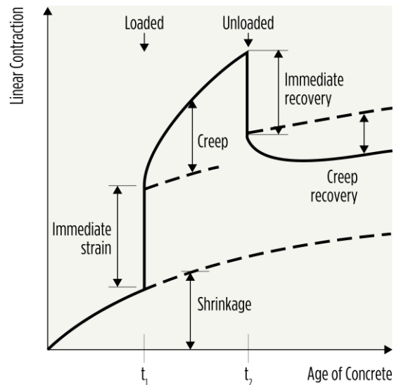
Figure 25.25 – Creep Deformation of Concrete
