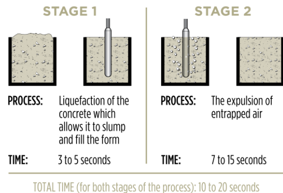
Figure 13.1 – The Process of Compaction
