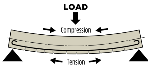
Figure 1.12 – Simply Supported Beams or Slabs
