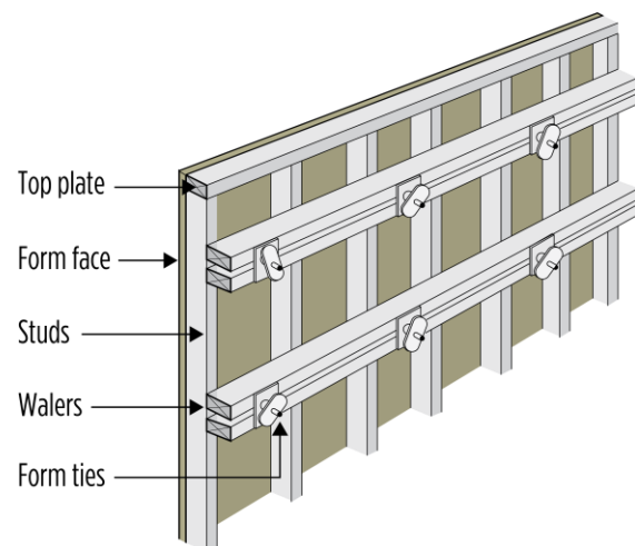
Figure 27.1 – Wall Forms
