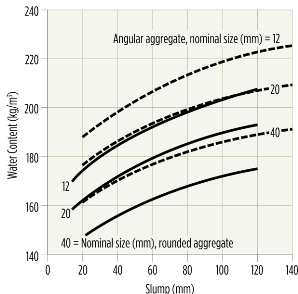
Figure 3.2 – Water Requirement for Concrete using Aggregates of Different Shapes and Nominal Sizes
