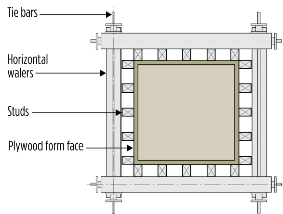
Figure 27.3 – Column Forms
