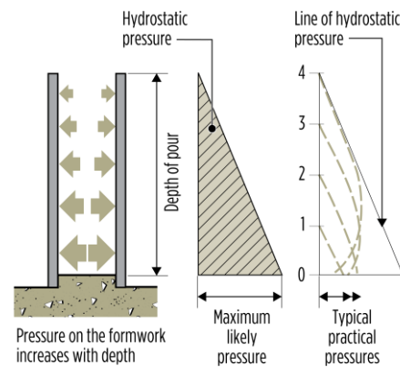
Figure 27.13 - Lateral Pressures on Formwork during Compaction
