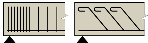
Figure 1.11 – Reinforcement to Resist Diagonal Tension
