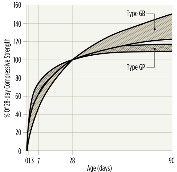
Figure 25.20 – Concrete Strength Development – Type GP and Type GB Cements
